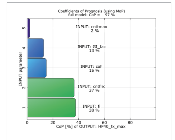
Figure 8: Coefficients of prognosis – highest hammer position
