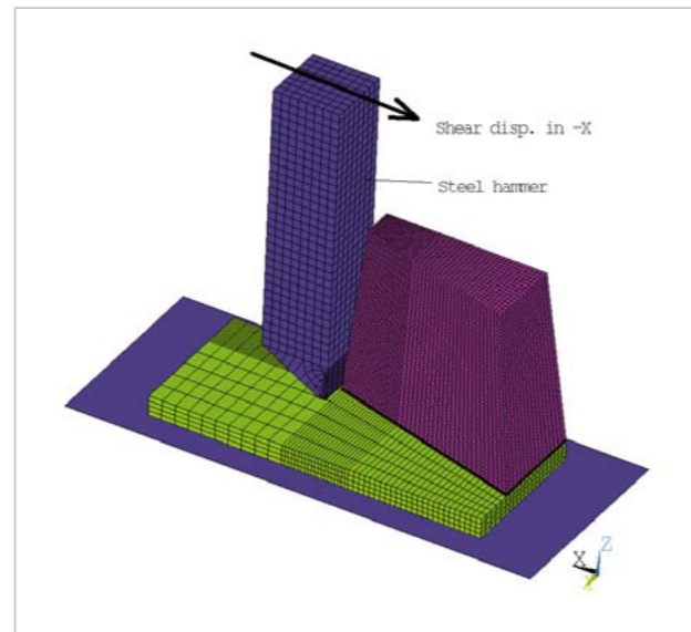
Fig. 1: Steel hammer with shearing direction
