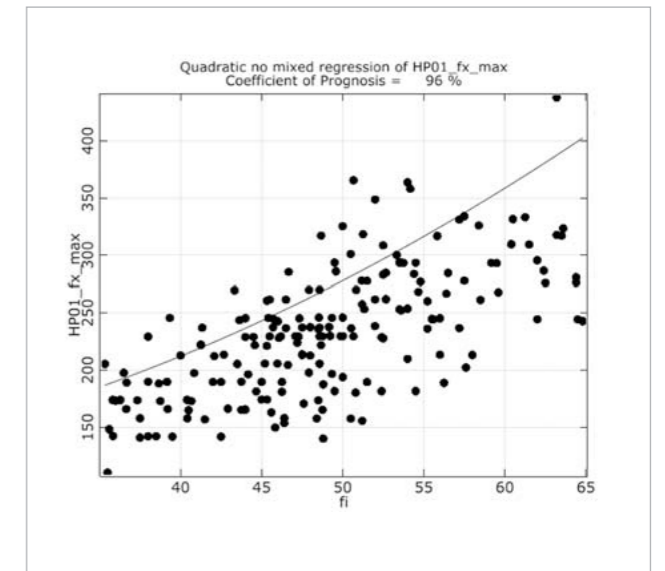
Fig. 7: Anthill plot – lowest hammer position
