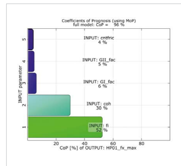
Fig. 6: Coefficients of prognosis – lowest hammer position
