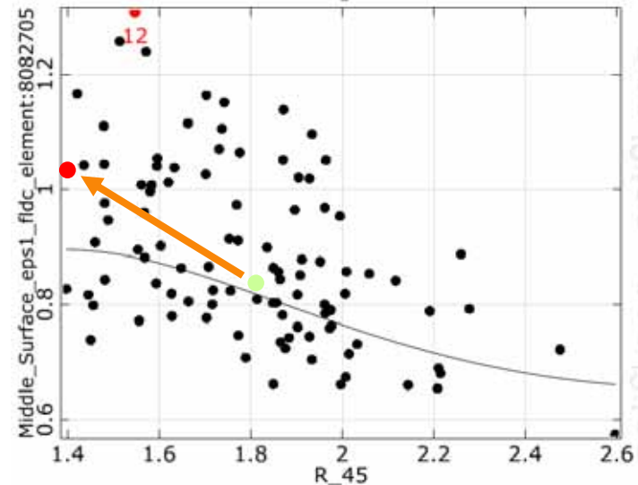
MLS approximation of Middle_Surface_eps1_fldc_element:8082705 Coefficient of Prognosis = 44 %
