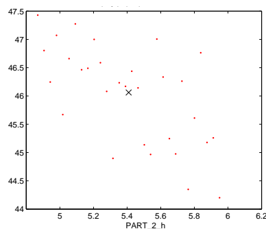
Figure 5: r_{XY} \approx -0.63
