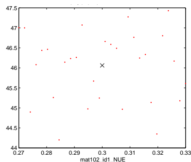
Figure 6: r_{XY} \approx -0.03
