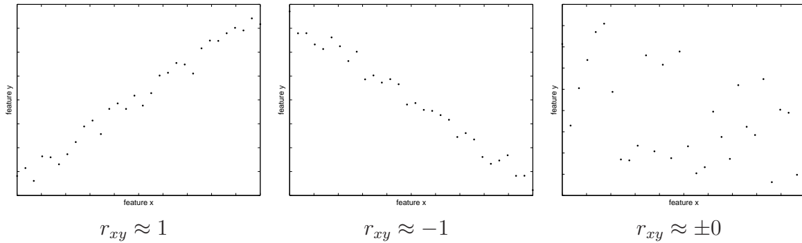
Figure 1: different correlations of two features
